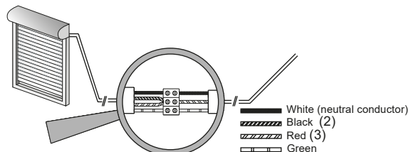
Fig. 7 Radio connection (transmitter operation)
